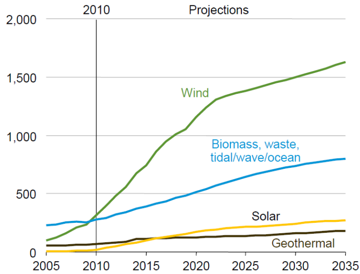
Figure 4: World Renewable Electricity Generation by Source, forecasted to 2035
